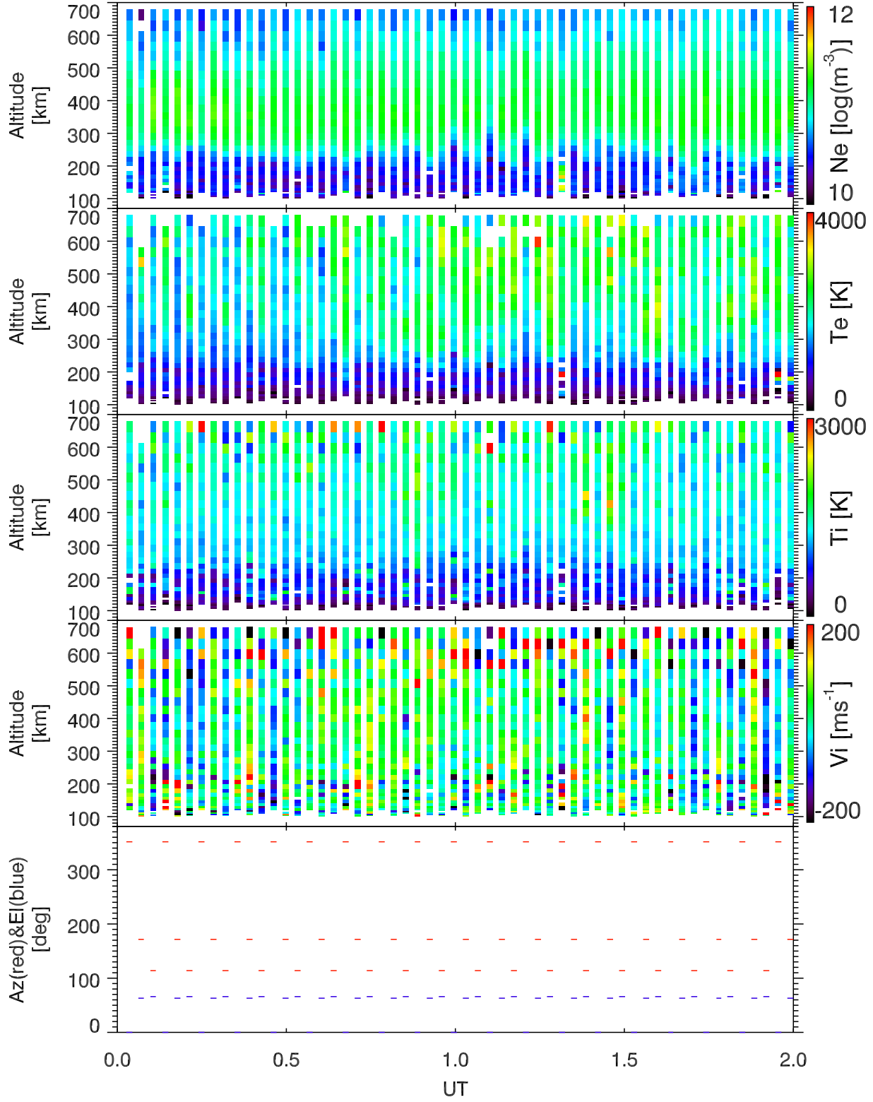
EISCAT 2002-11-12_00_02UT_tau0_ant@32m.
