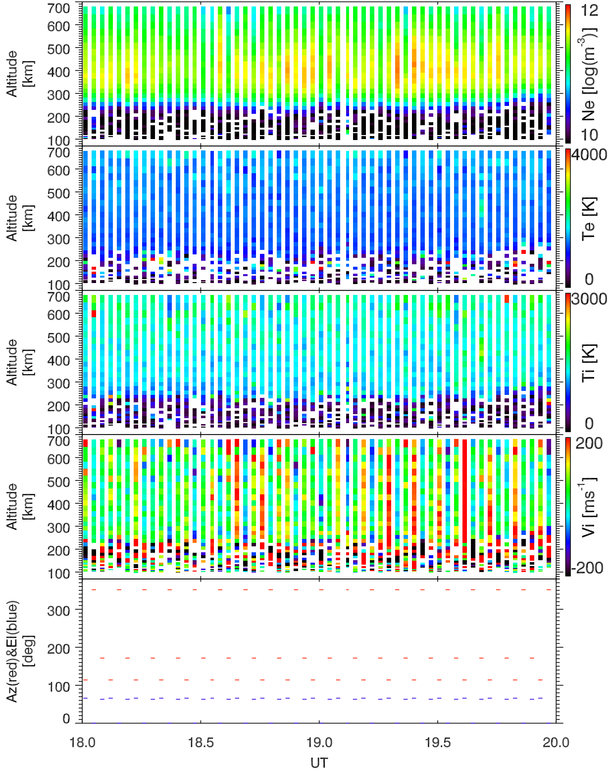
EISCAT 2002-11-12_18_20UT_tau0_ant@32m.
