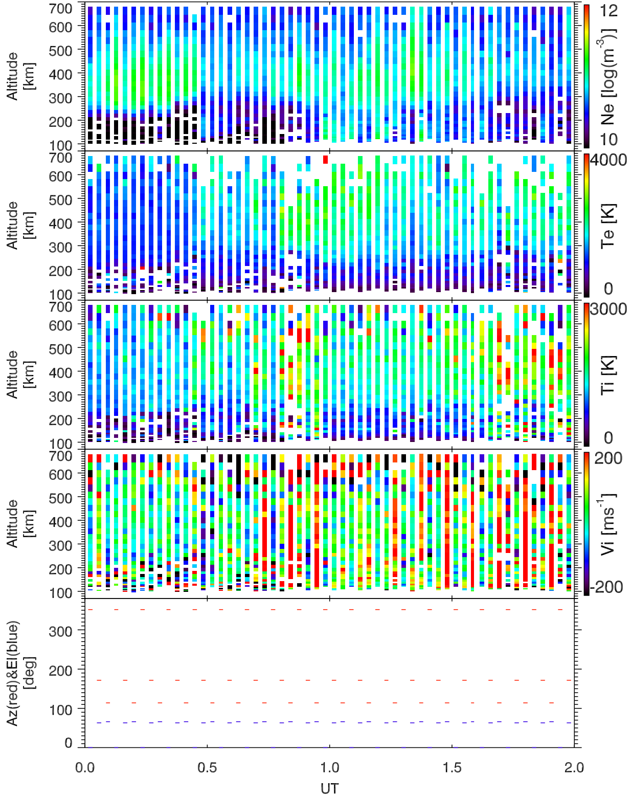
EISCAT 2002-11-14_00_02UT_tau0_ant@32m.
