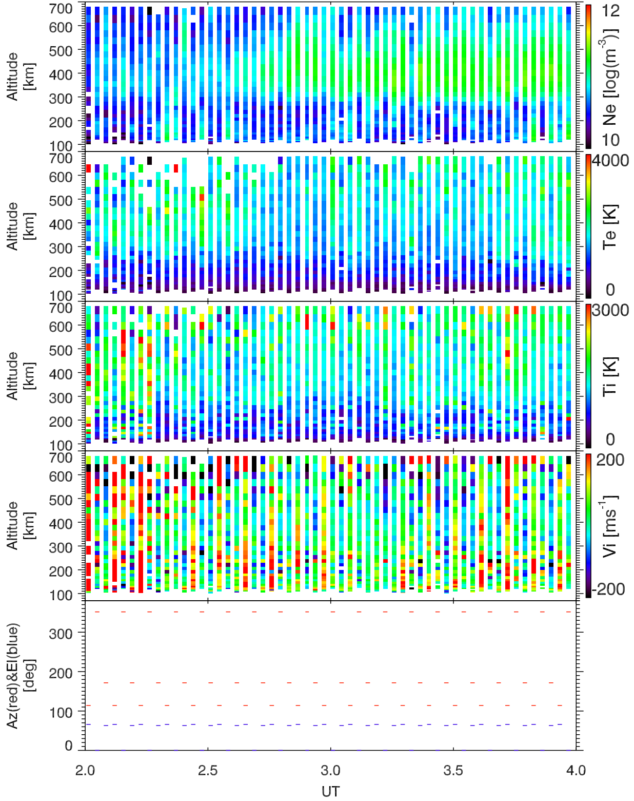
EISCAT 2002-11-14_02_04UT_tau0_ant@32m.
