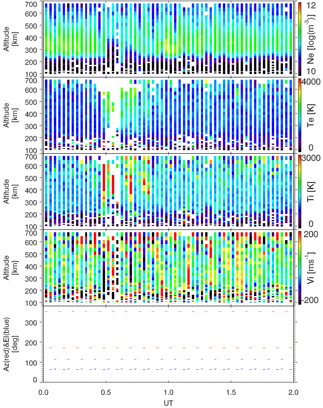
EISCAT 2002-11-15_00_02UT_tau0_ant@32m.
