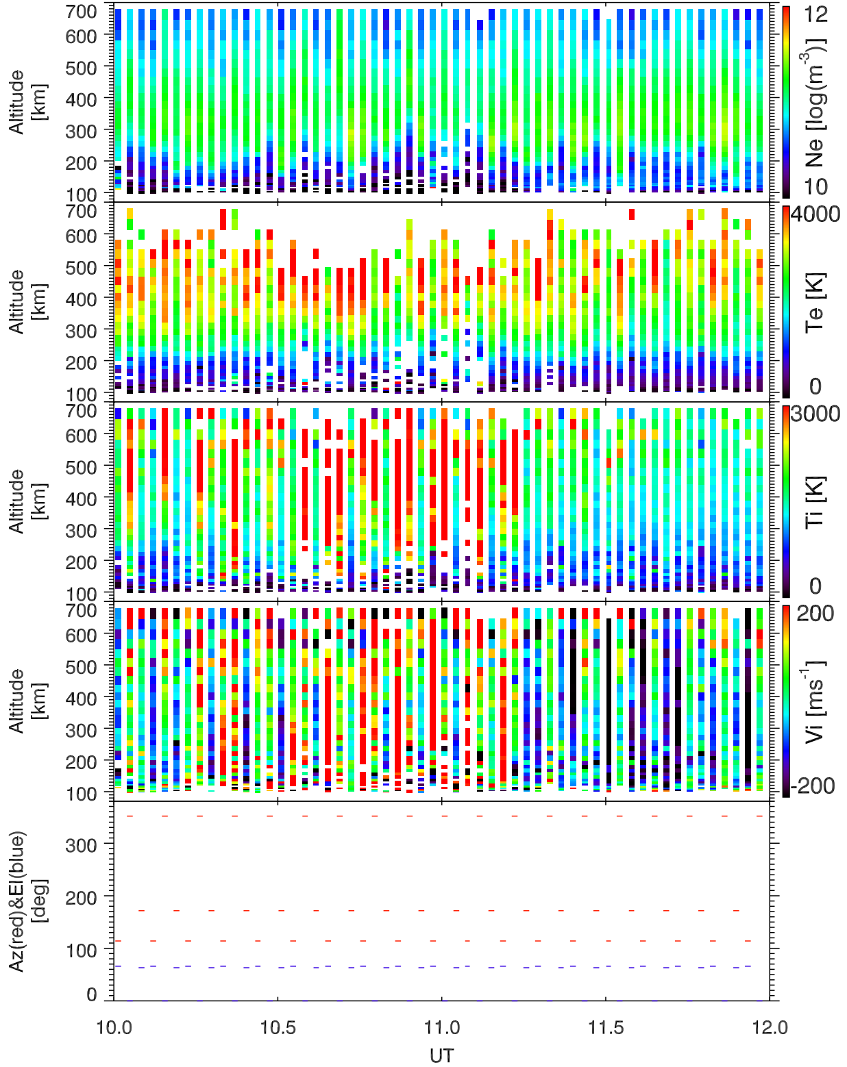
EISCAT 2002-11-15_10_12UT_tau0_ant@32m.
