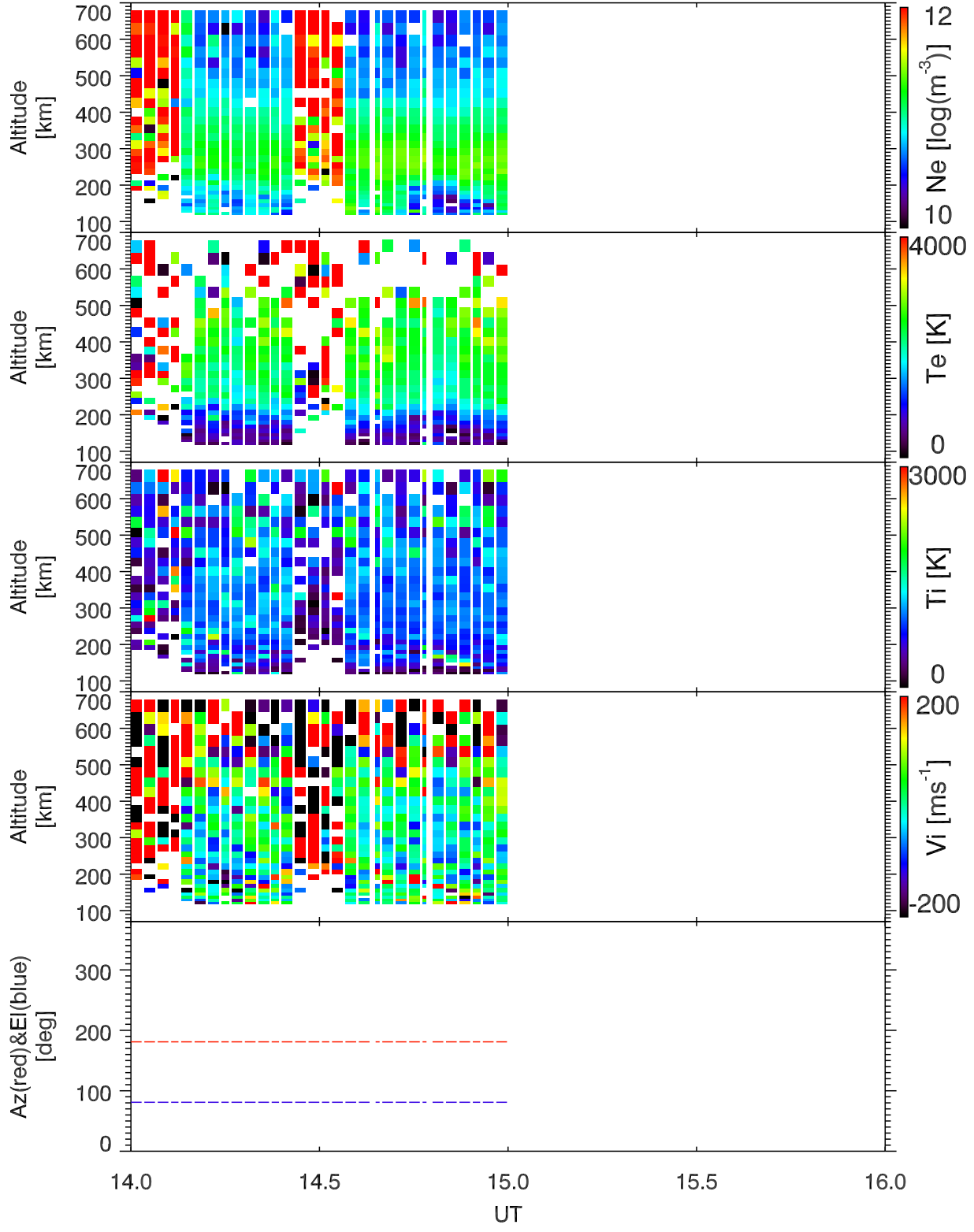
EISCAT 2003-02-24_14_16UT_tau0_120@42m.
