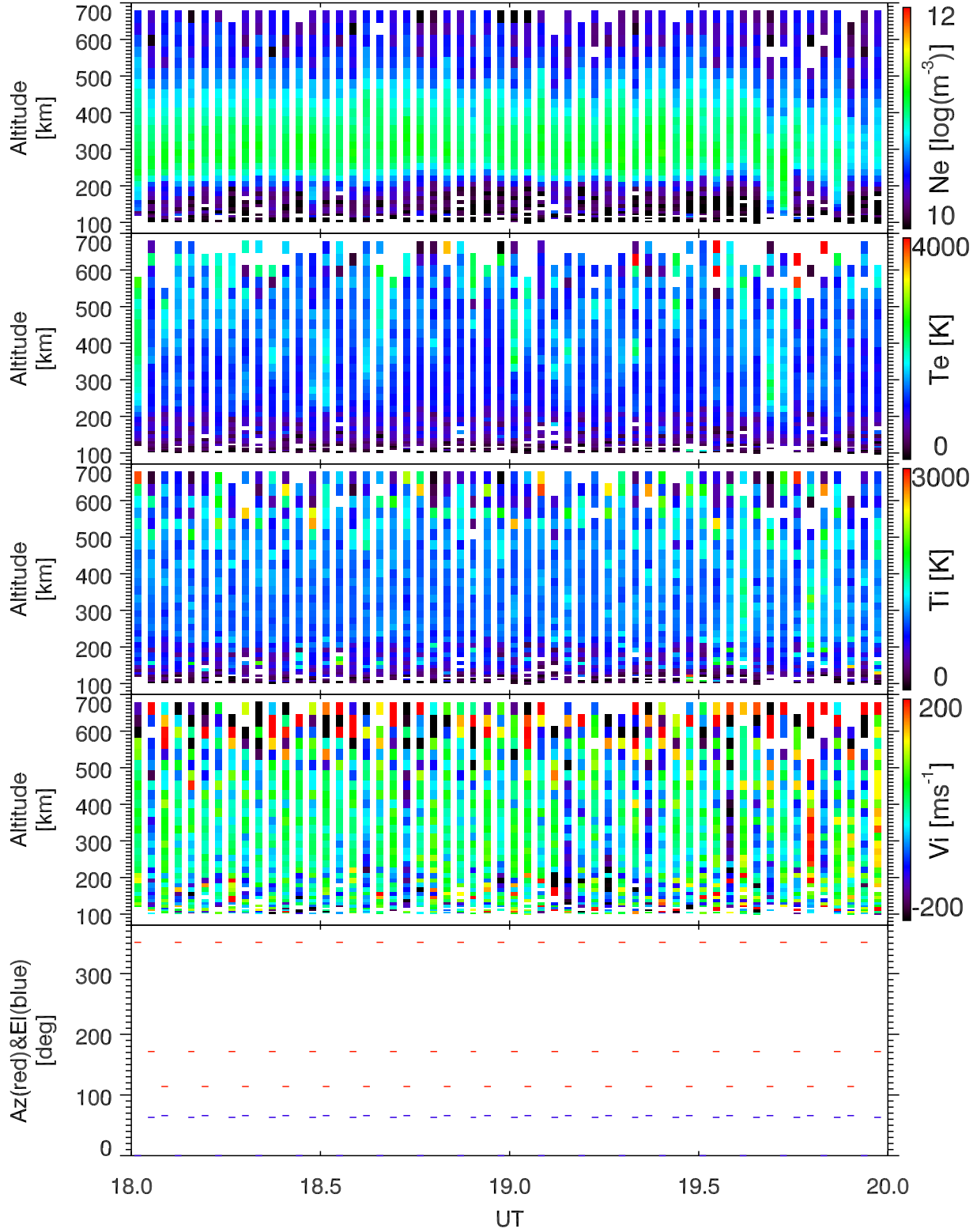
EISCAT 2003-02-24_18_20UT_tau0_ant@32m.
