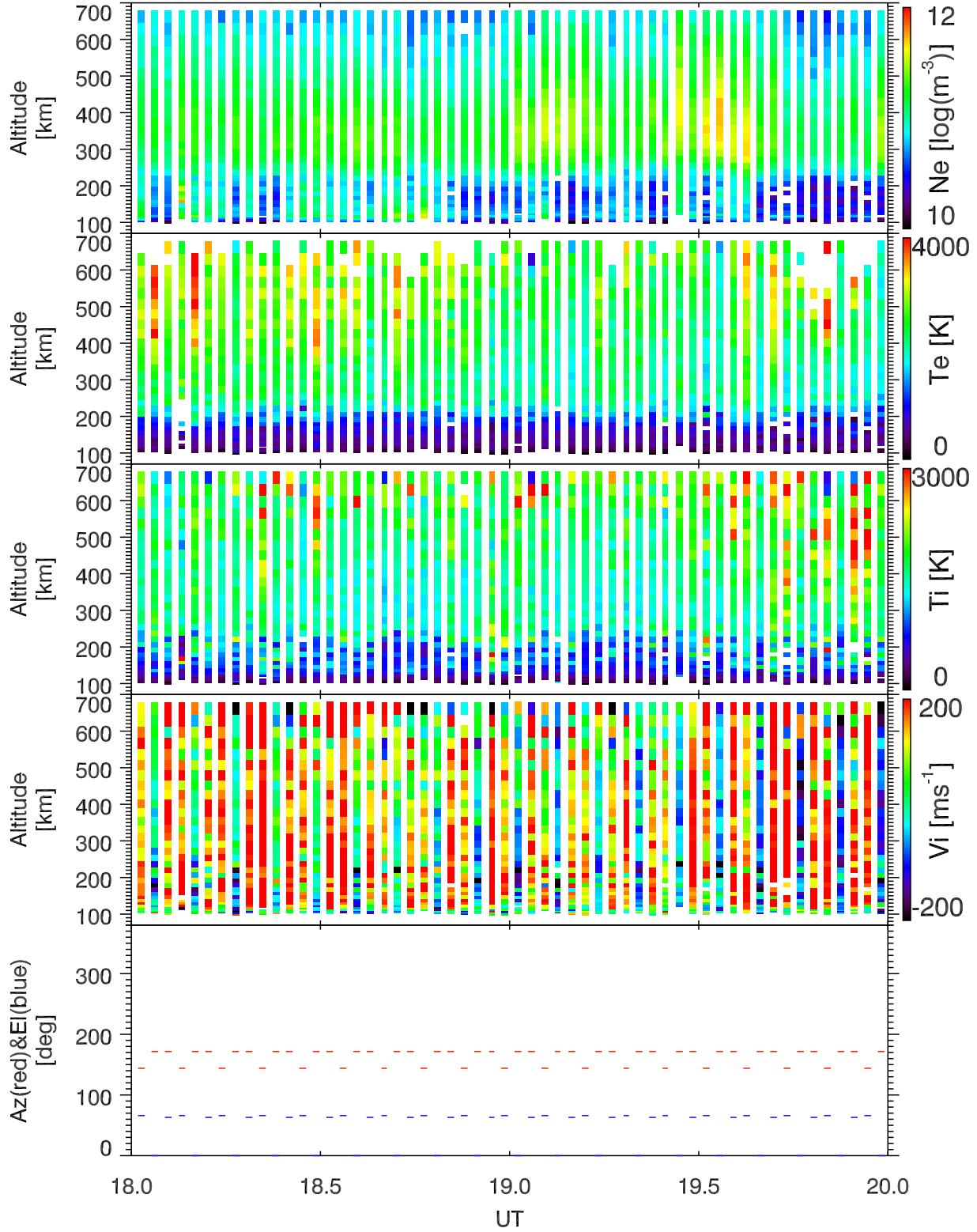
EISCAT 2003-03-20_18_20UT_tau0_ant@32m.
