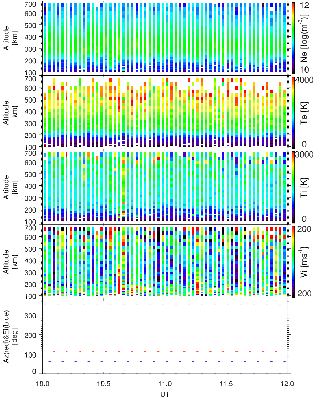
EISCAT 2003-10-30_10_12UT_tau0_ant@32m.
