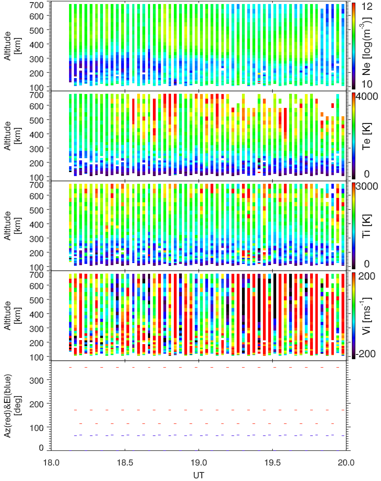
EISCAT 2003-10-30_18_20UT_tau0_ant@32m.
