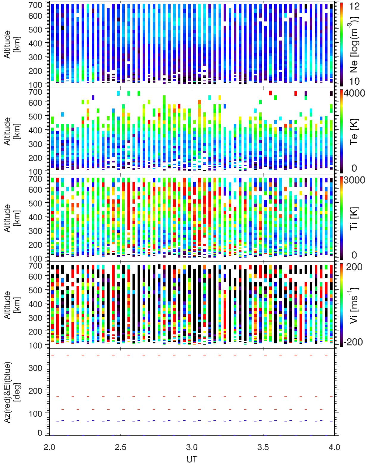
EISCAT 2003-10-31_02_04UT_tau0_ant@32m.
