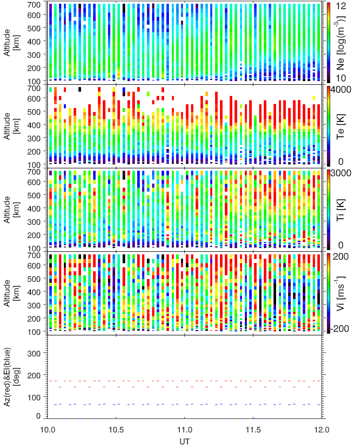
EISCAT 2003-10-31_10_12UT_tau0_ant@32m.
