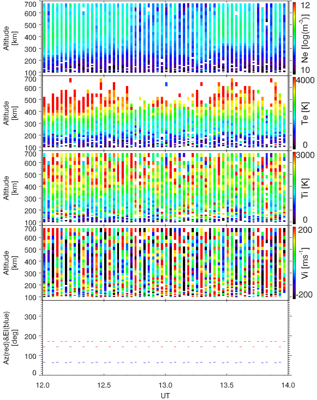
EISCAT 2003-10-31_12_14UT_tau0_ant@32m.
