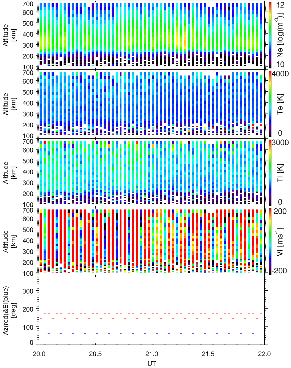
EISCAT 2003-11-01_20_22UT_tau0_ant@32m.
