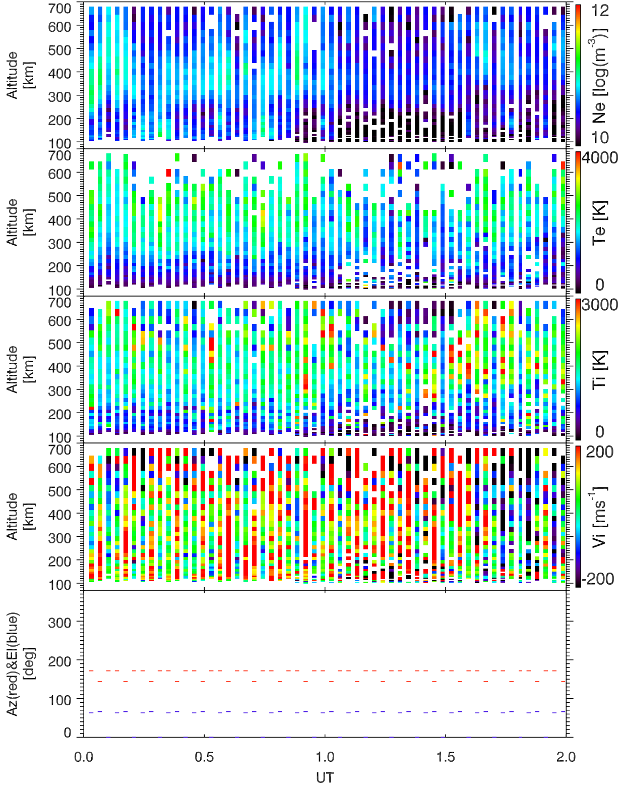
EISCAT 2003-11-02_00_02UT_tau0_ant@32m.
