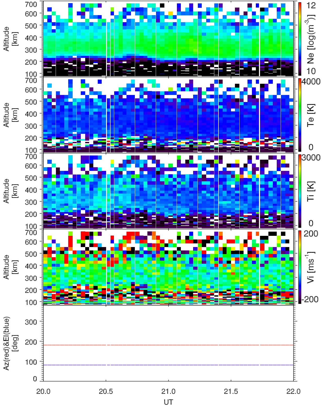
EISCAT 2004-02-19_20_22UT_steffe_120@42m.
