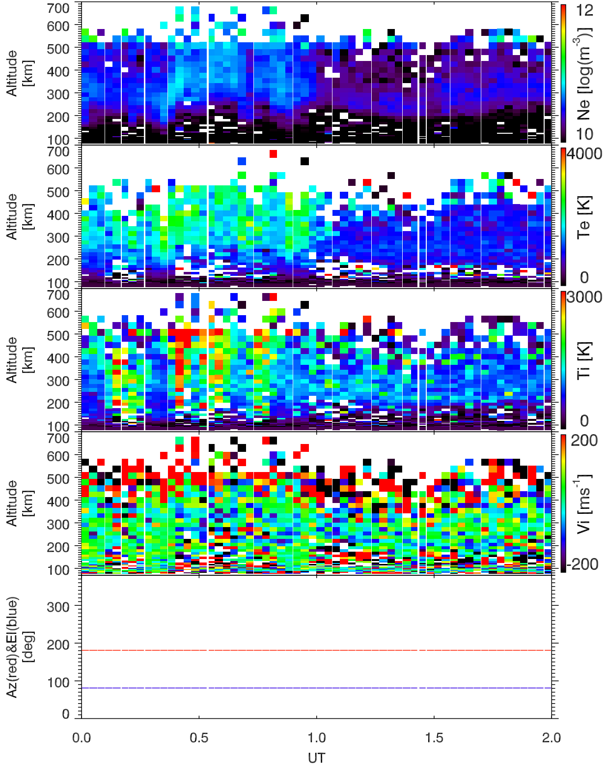
EISCAT 2004-02-20_00_02UT_steffe_120@42m.
