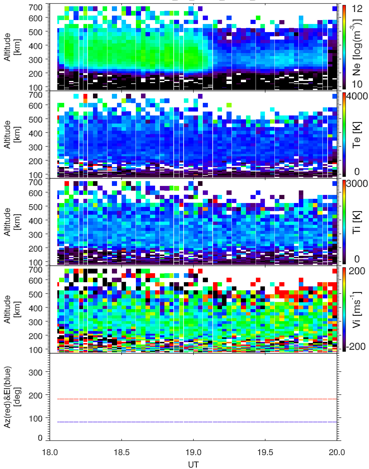
EISCAT 2004-02-20_18_20UT_steffe_120@42m.
