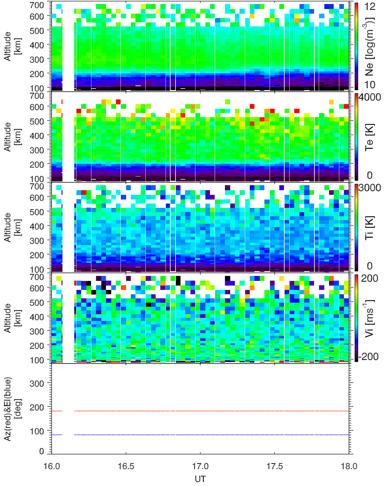
EISCAT 2004-03-30_16_18UT_steffe_120@42m.
