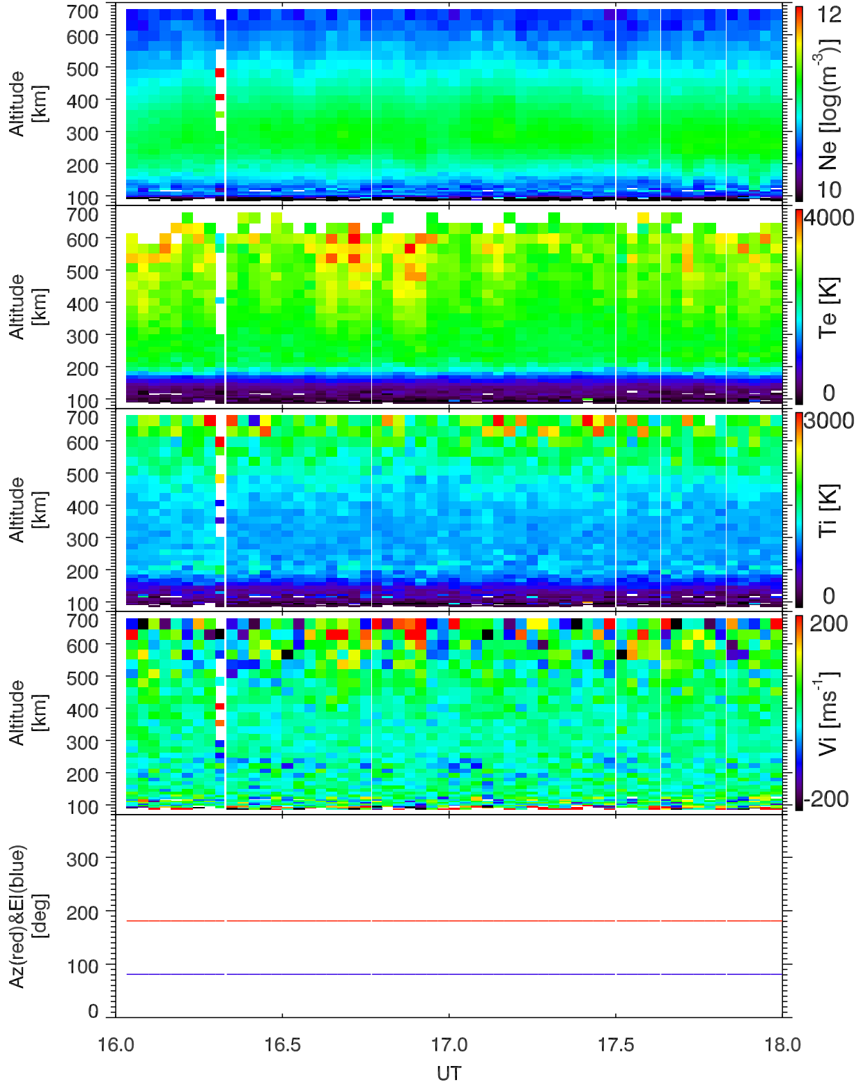
EISCAT 2004-06-01_16_18UT_tau0_120@42m.
