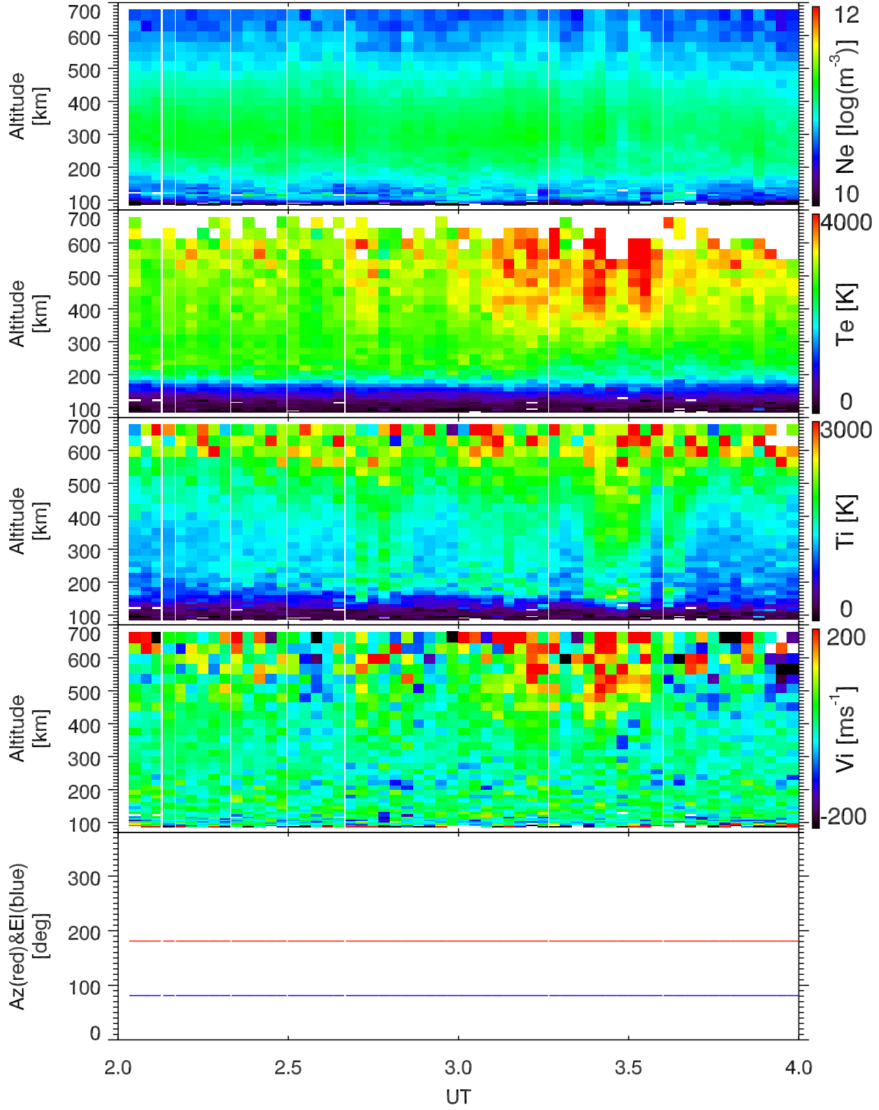
EISCAT 2004-06-02_02_04UT_tau0_120@42m.
