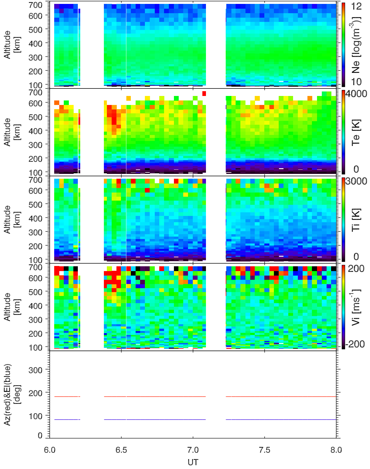
EISCAT 2004-06-03_06_08UT_tau0_120@42m.
