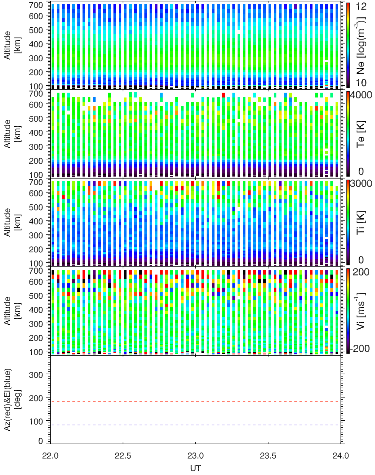
EISCAT 2004-06-04_22_24UT_all_all@42m.
