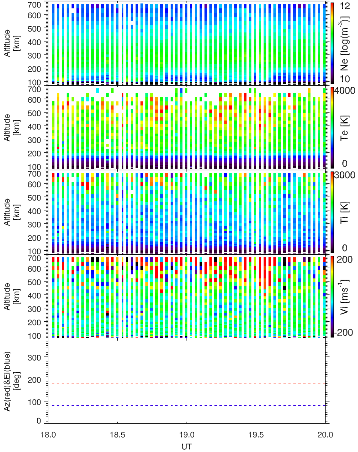
EISCAT 2004-06-07_18_20UT_steffe_ant@42m.
