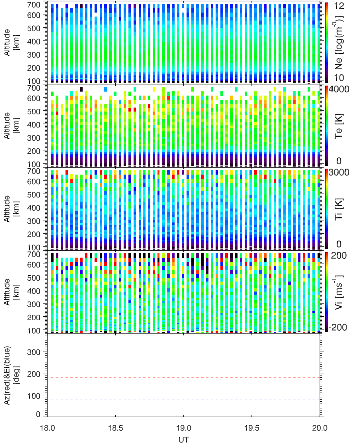
EISCAT 2004-06-08_18_20UT_steffe_ant@42m.
