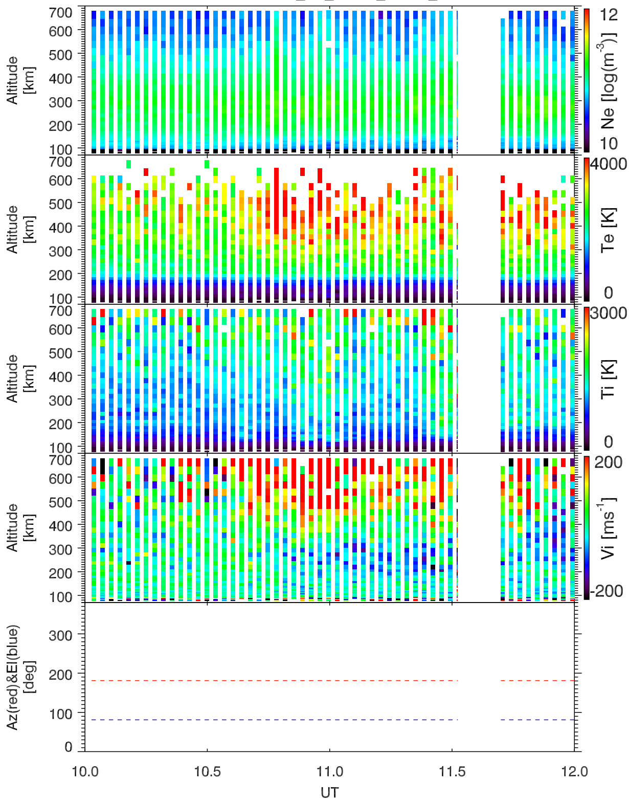
EISCAT 2004-06-09_10_12UT_steffe_ant@42m.
