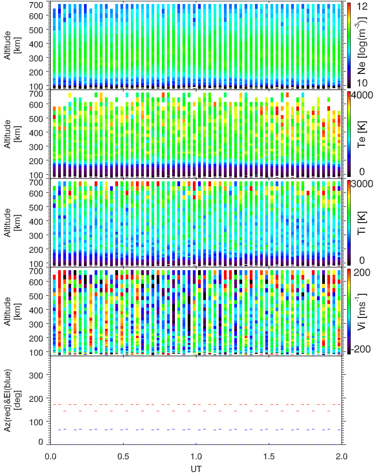
EISCAT 2004-06-14_00_02UT_steffe_ant@32m.
