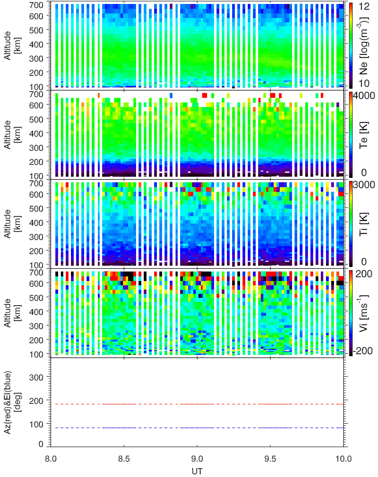
EISCAT 2005-04-19_08_10UT_tau0_all@42m.
