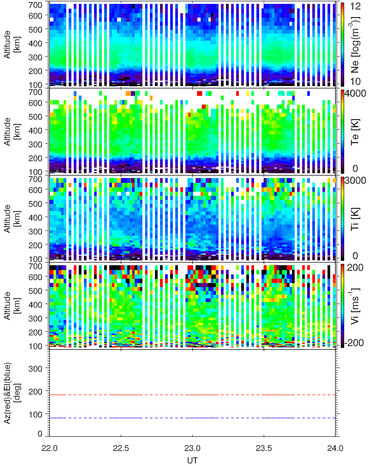
EISCAT 2005-04-20_22_24UT_tau0_all@42m.
