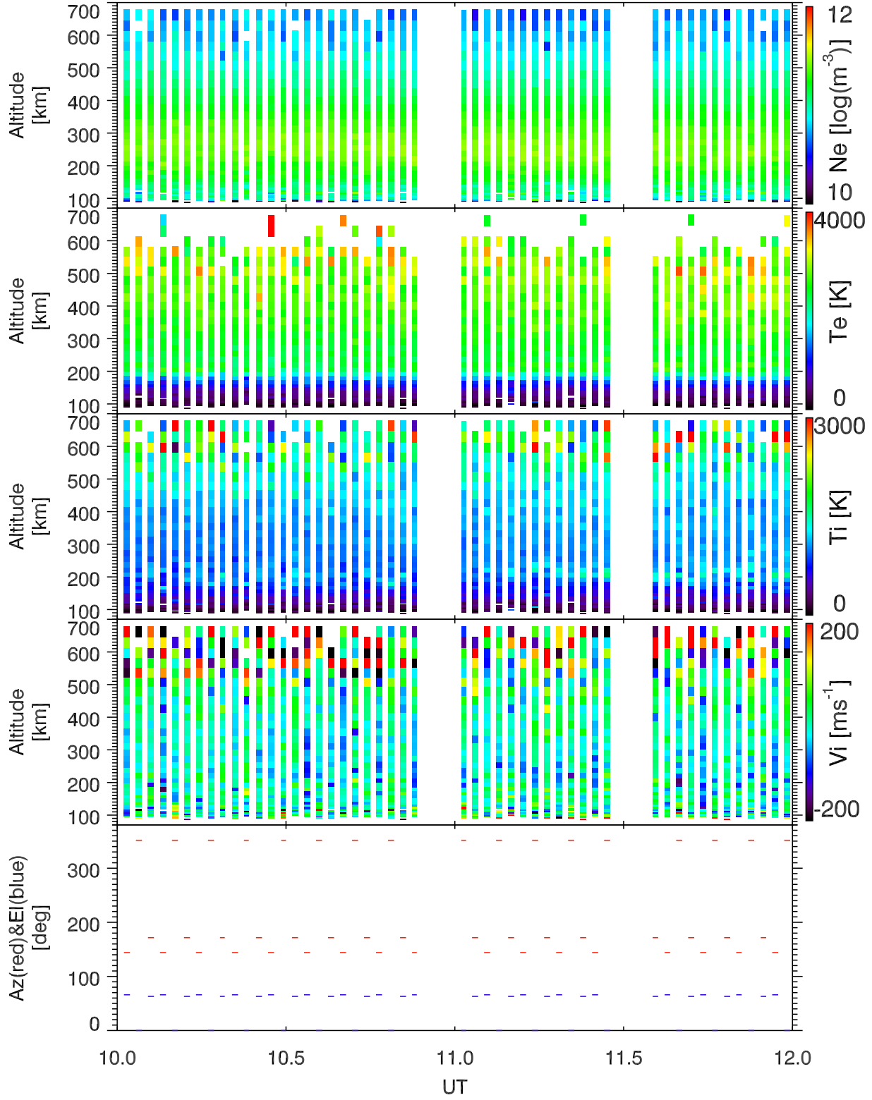
EISCAT 2005-07-01_10_12UT_tau0_ant@32m.
