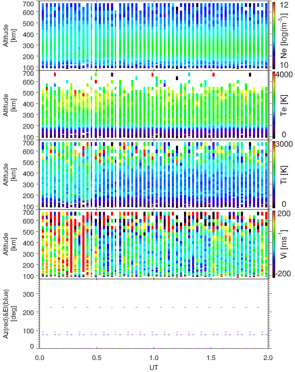
EISCAT 2005-07-23_00_02UT_tau0_ant@32m.
