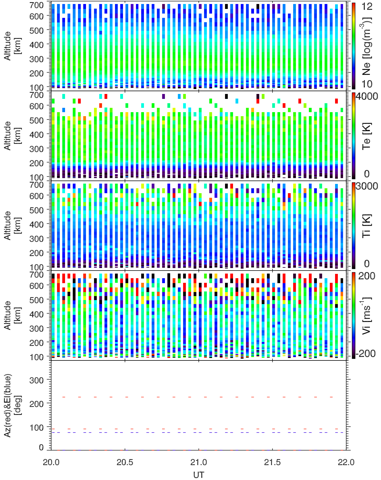
EISCAT 2005-07-23_20_22UT_tau0_ant@32m.
