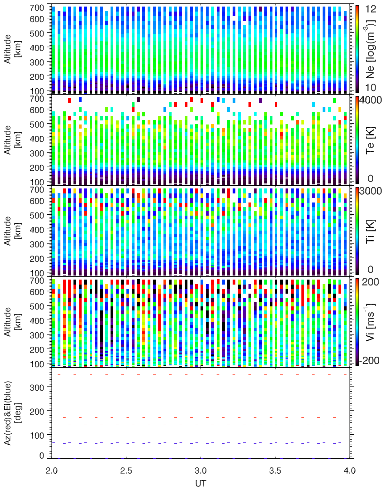
EISCAT 2005-09-02_02_04UT_steffe_ant@32m.
