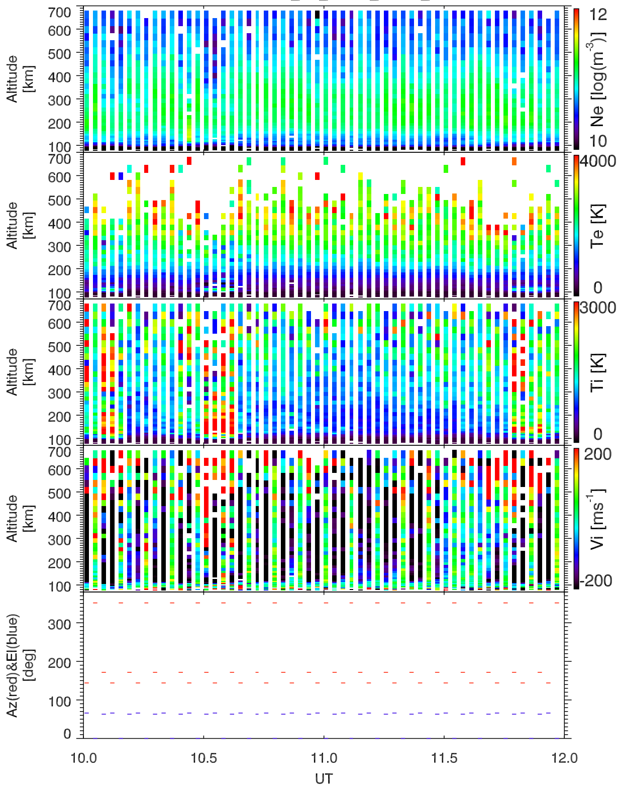
EISCAT 2005-09-03_10_12UT_steffe_ant@32m.
