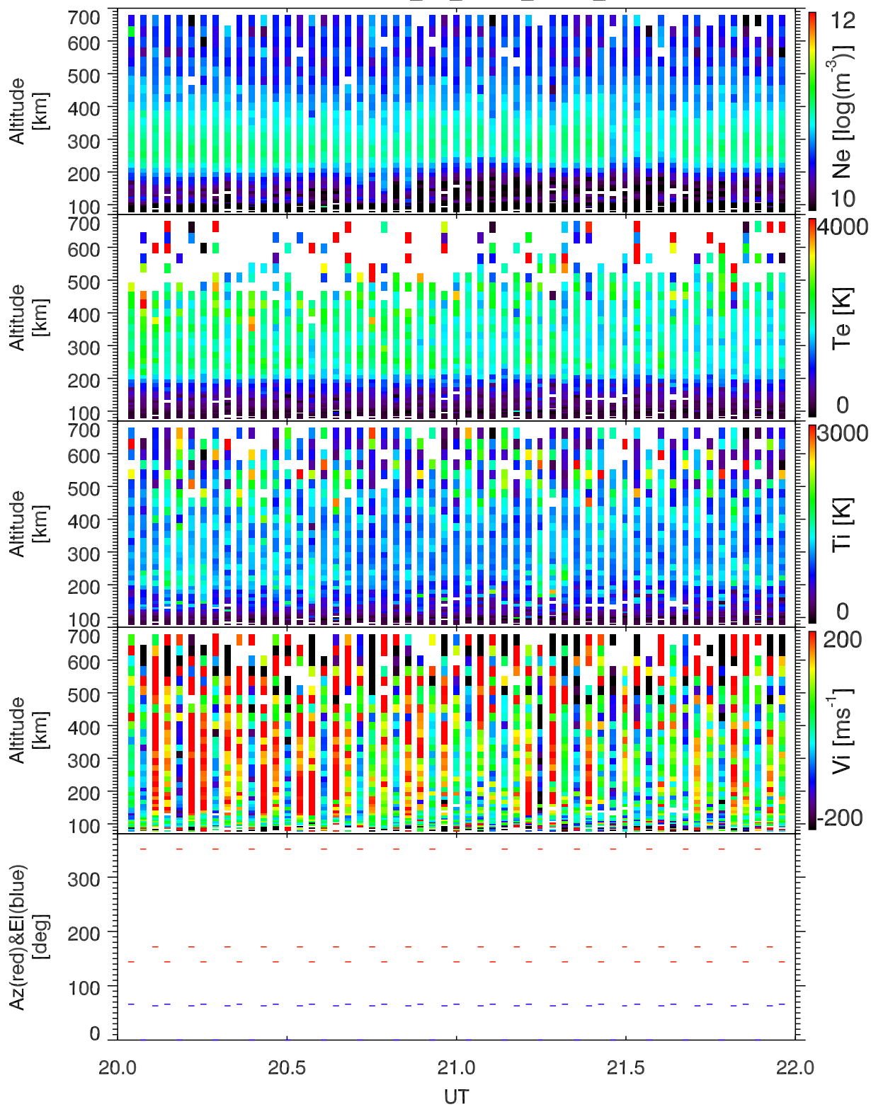
EISCAT 2005-09-03_20_22UT_steffe_ant@32m.
