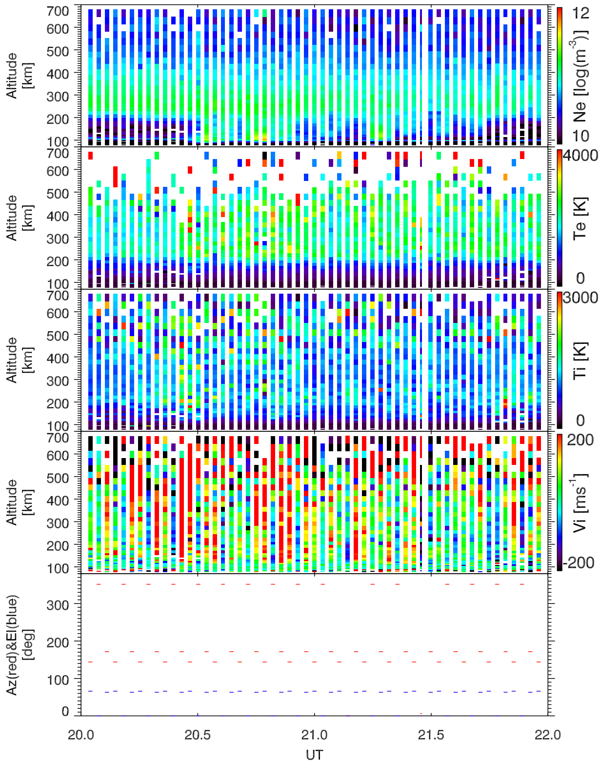
EISCAT 2005-09-05_20_22UT_steffe_ant@32m.
