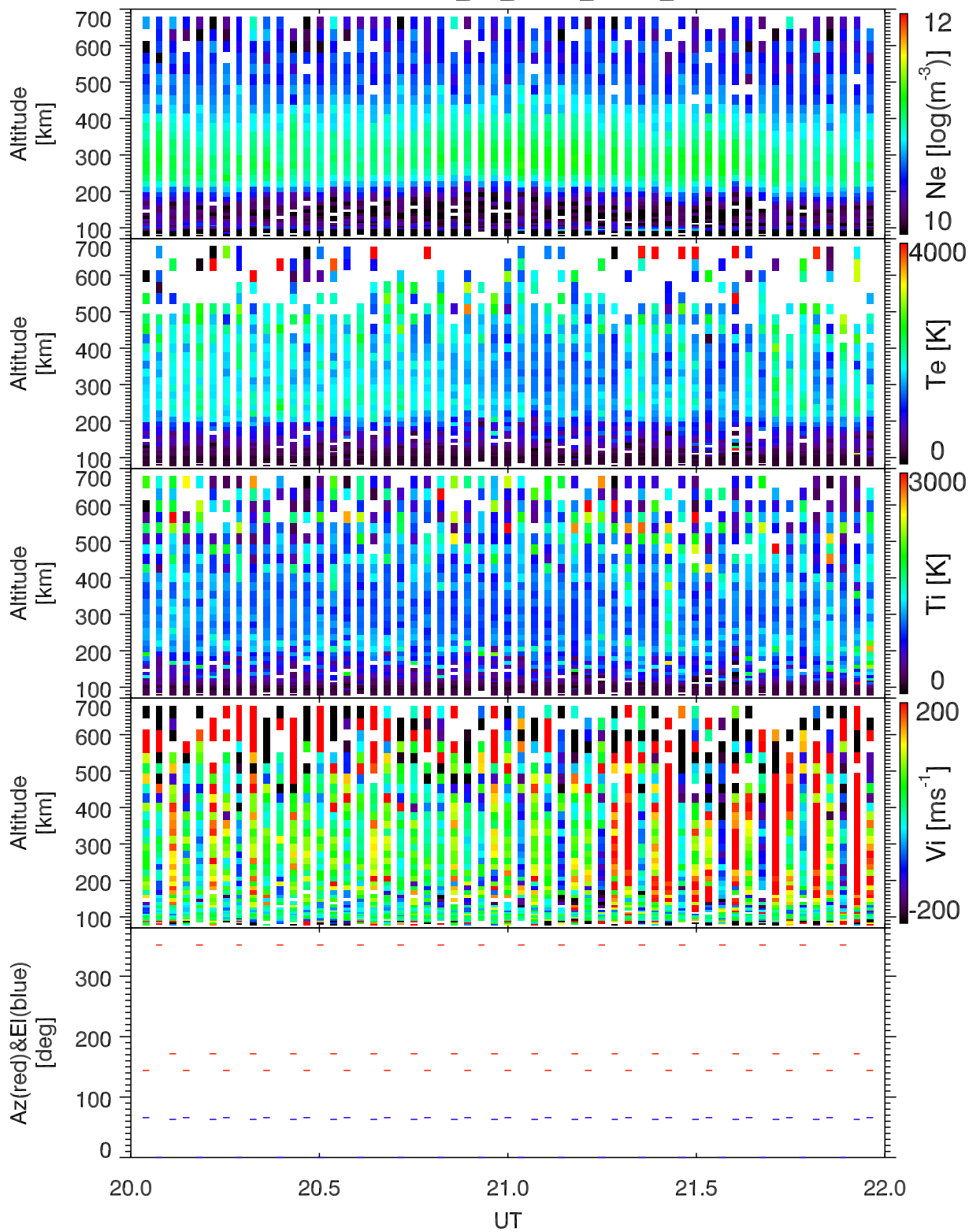
EISCAT 2005-09-06_20_22UT_steffe_ant@32m.
