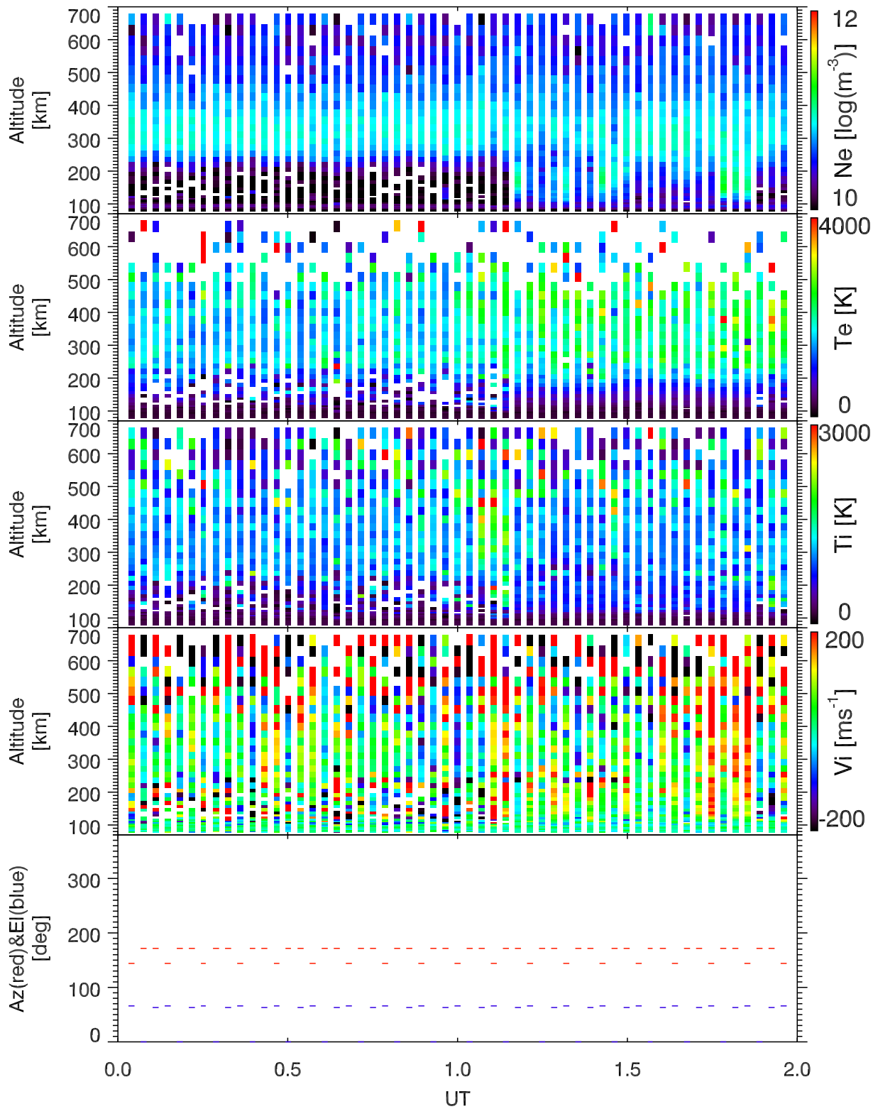
EISCAT 2005-09-15_00_02UT_steffe_ant@32m.
