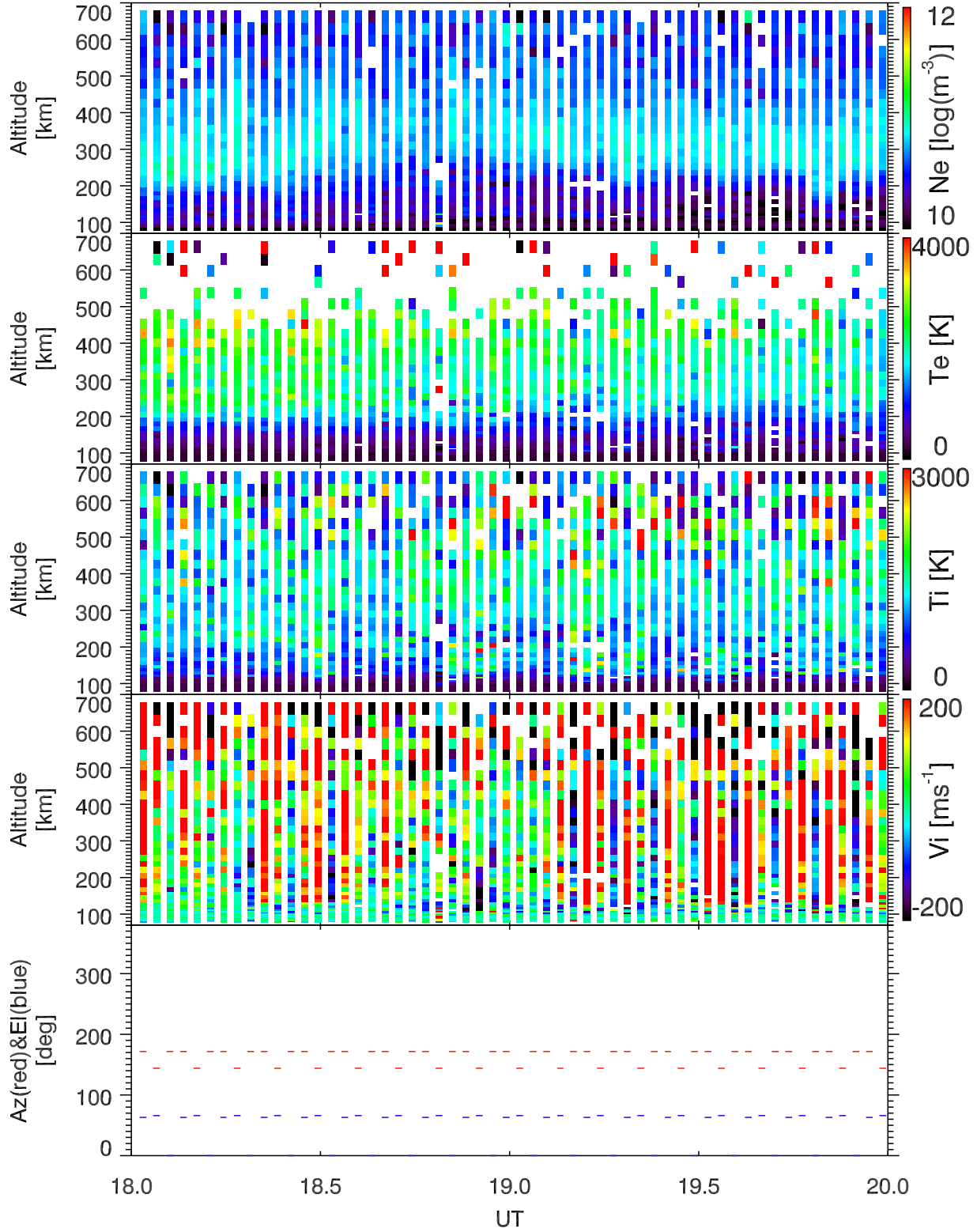
EISCAT 2005-09-15_18_20UT_steffe_ant@32m.
