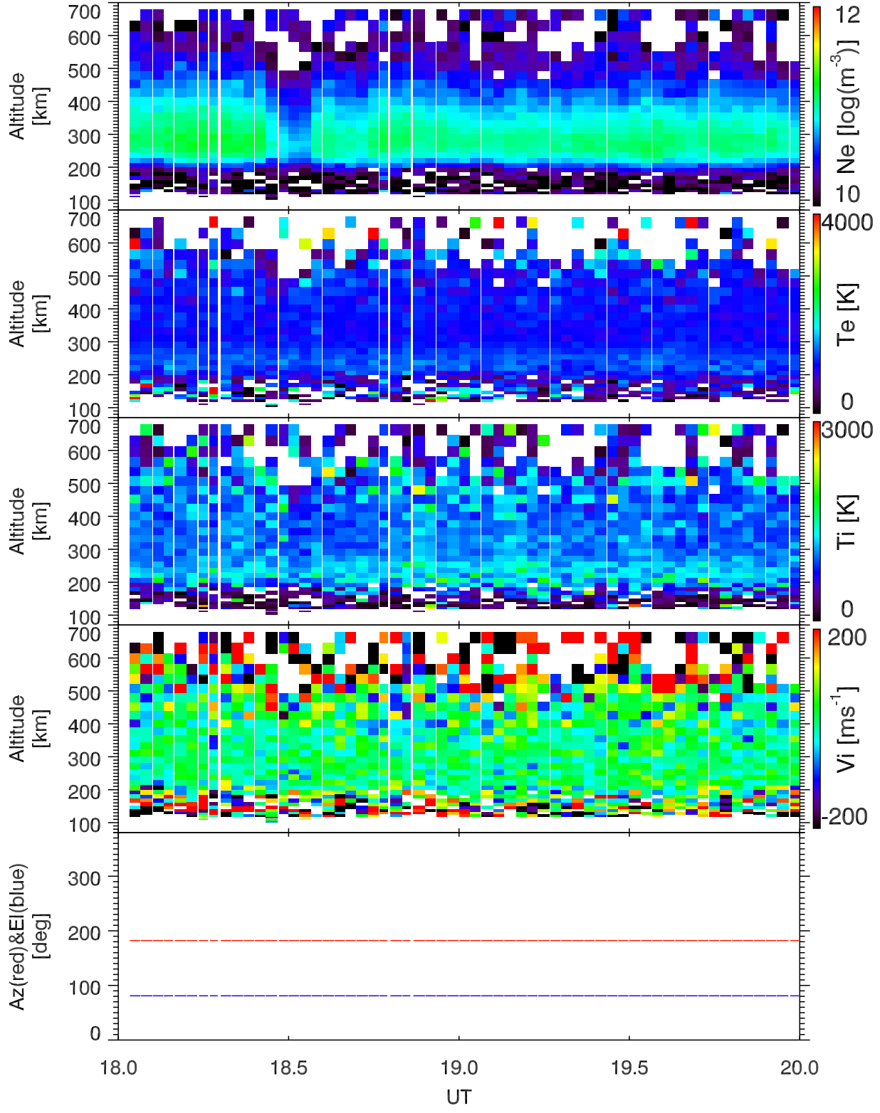
EISCAT 2005-10-17_18_20UT_tau0_120@42m.
