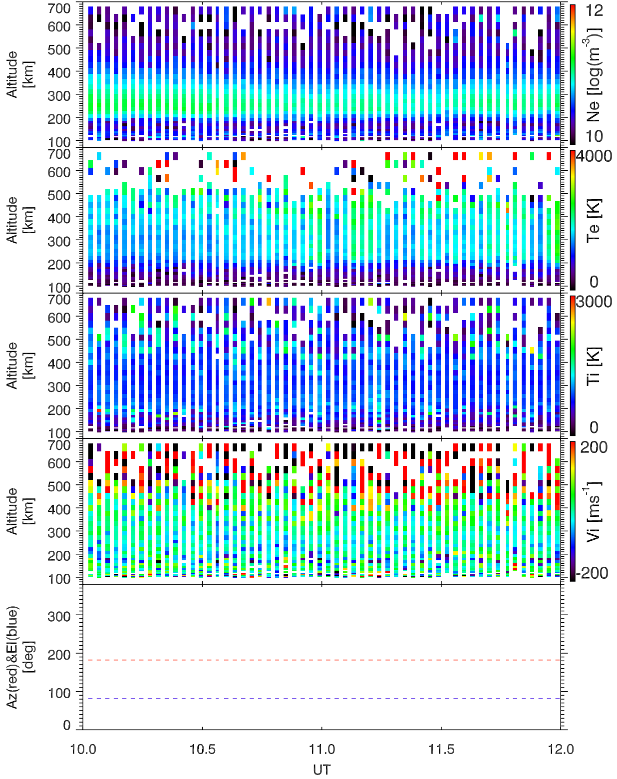
EISCAT 2005-11-08_10_12UT_tau0_ant@42m.
