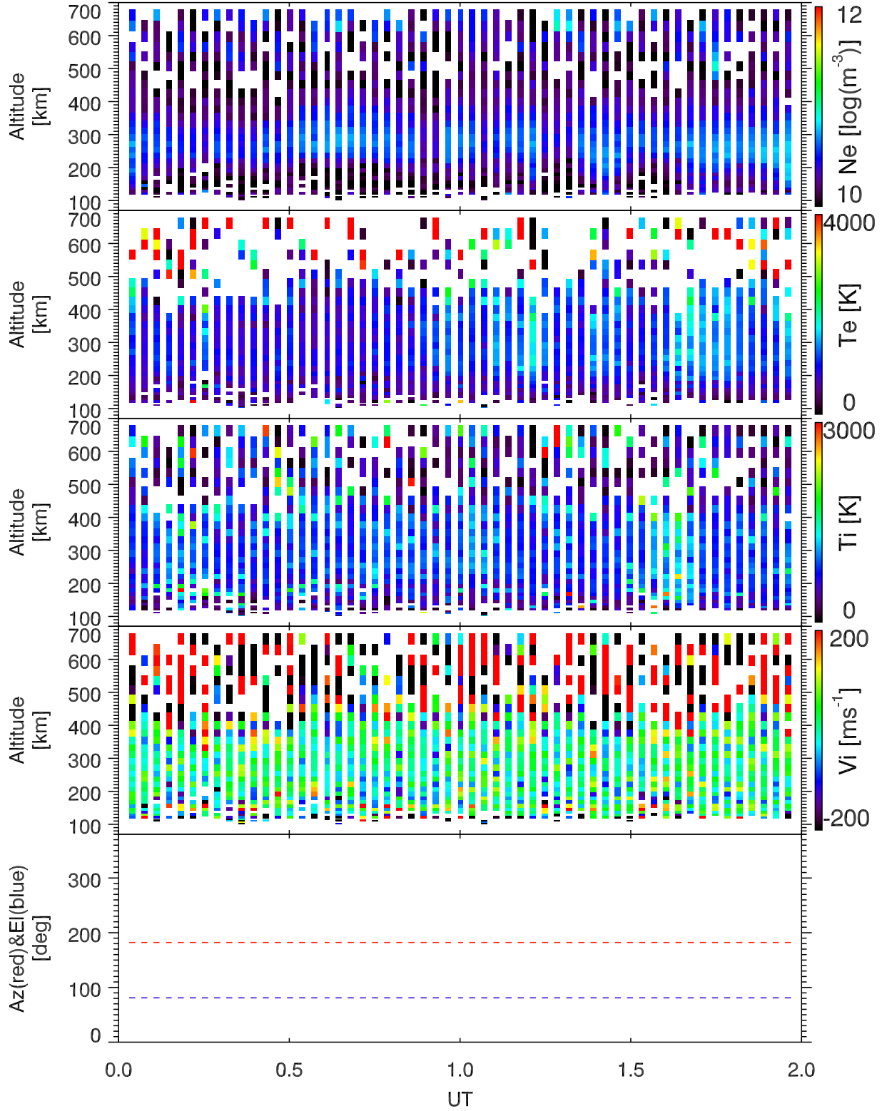
EISCAT 2005-11-09_00_02UT_tau0_ant@42m.
