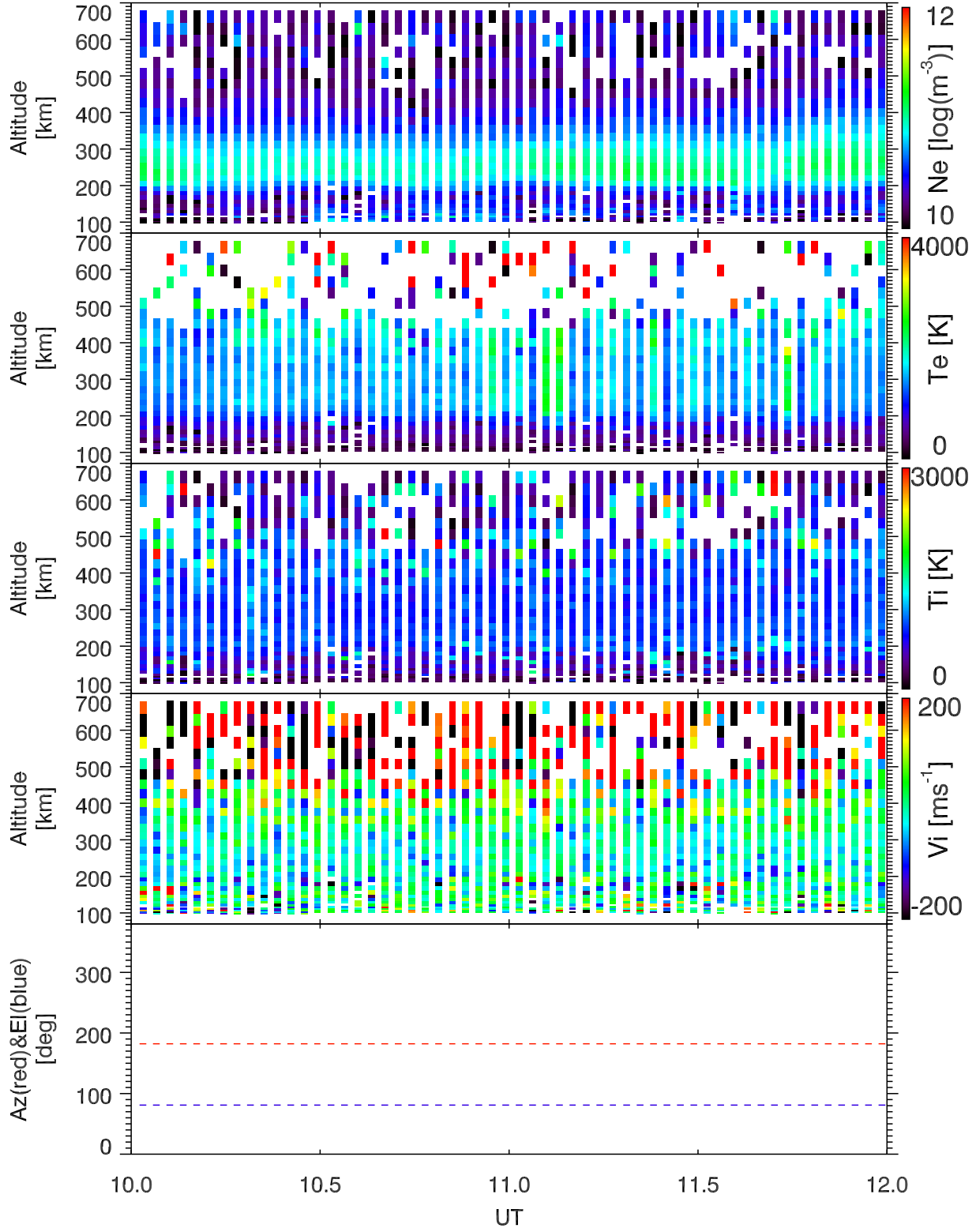
EISCAT 2005-11-10_10_12UT_tau0_ant@42m.
