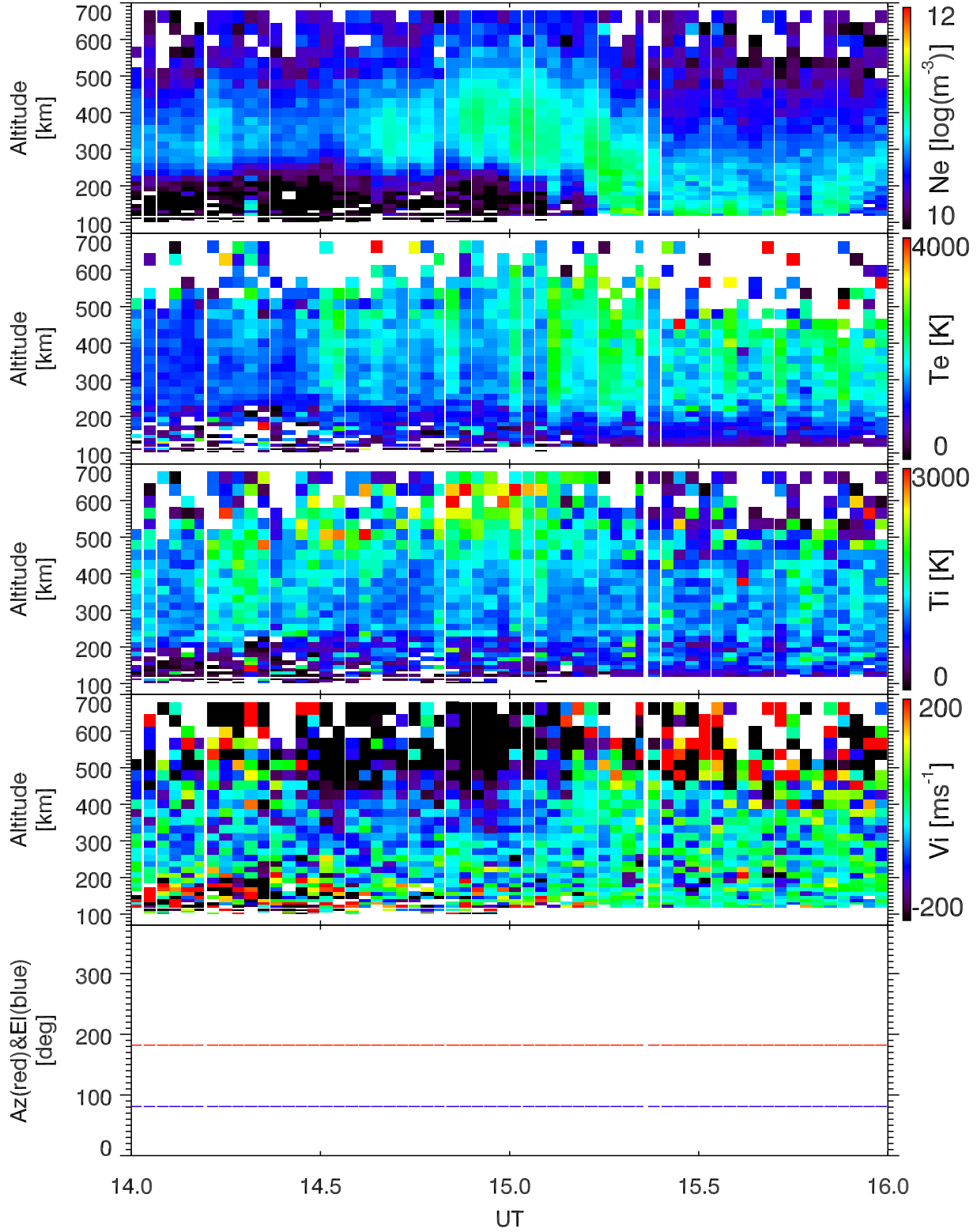
EISCAT 2005-12-18_14_16UT_tau0_all@42m.
