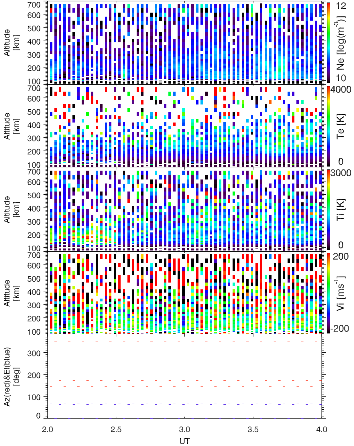
EISCAT 2007-02-07_02_04UT_steffe_ant@32m.
