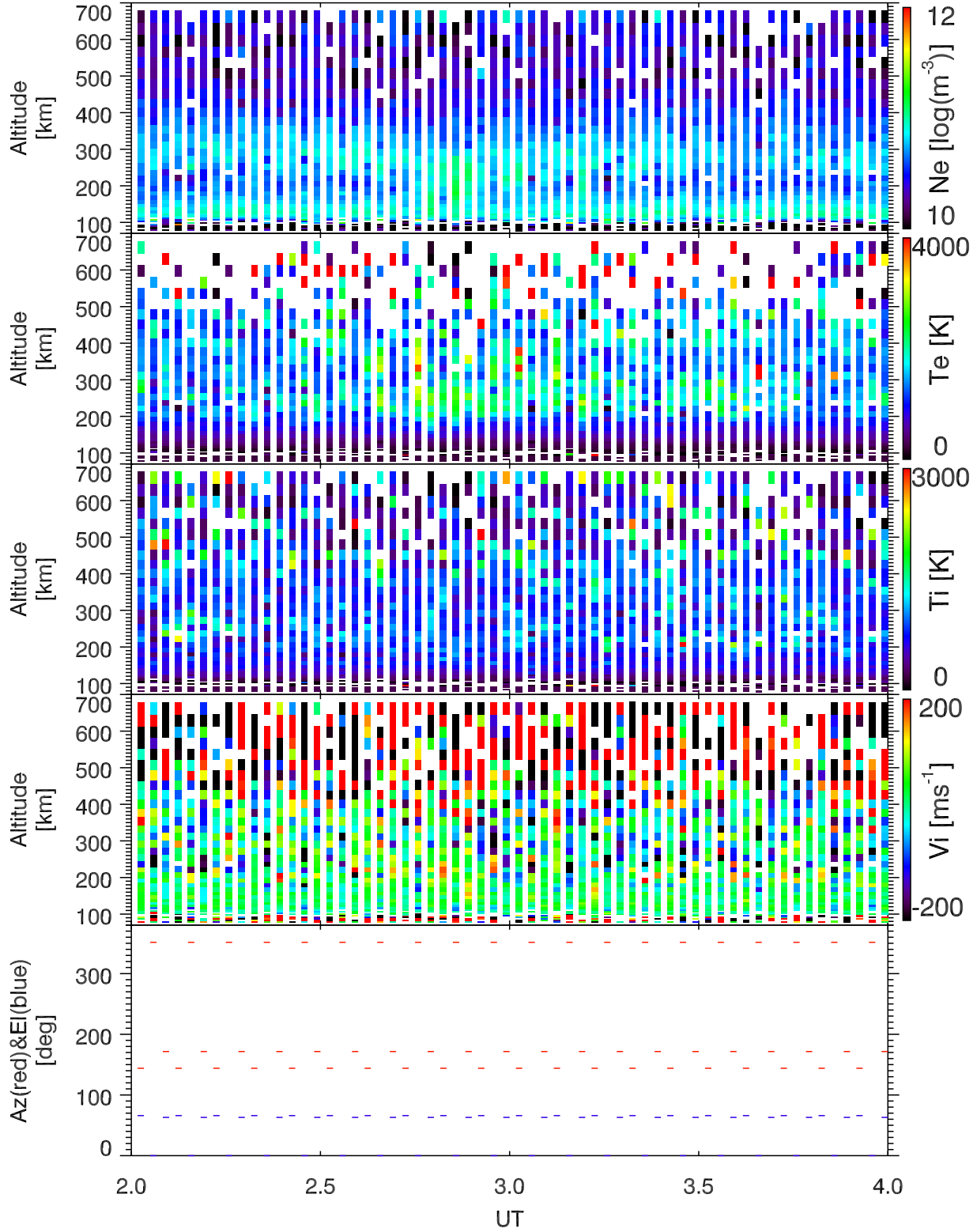
EISCAT 2007-03-05_02_04UT_steffe_ant@32m.
