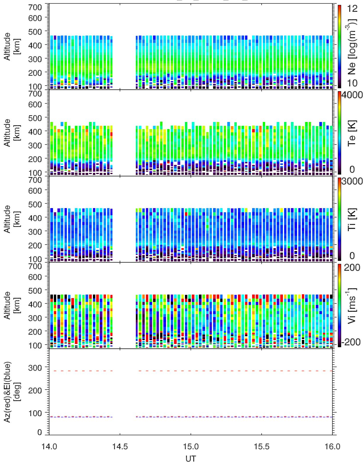
EISCAT 2007-03-20_14_16UT_ipy_ant@32m.
