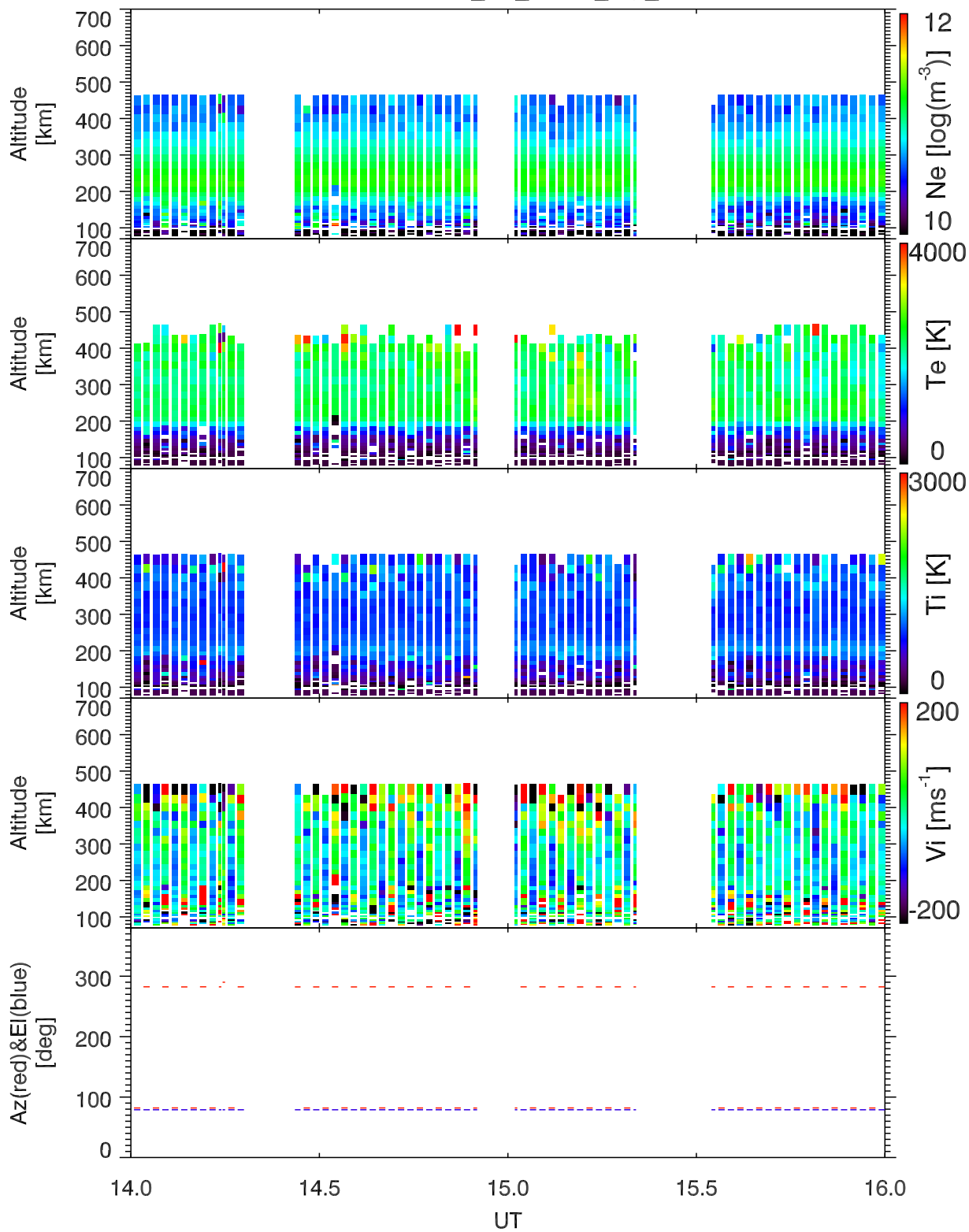
EISCAT 2007-03-21_14_16UT_ipy_ant@32m.
