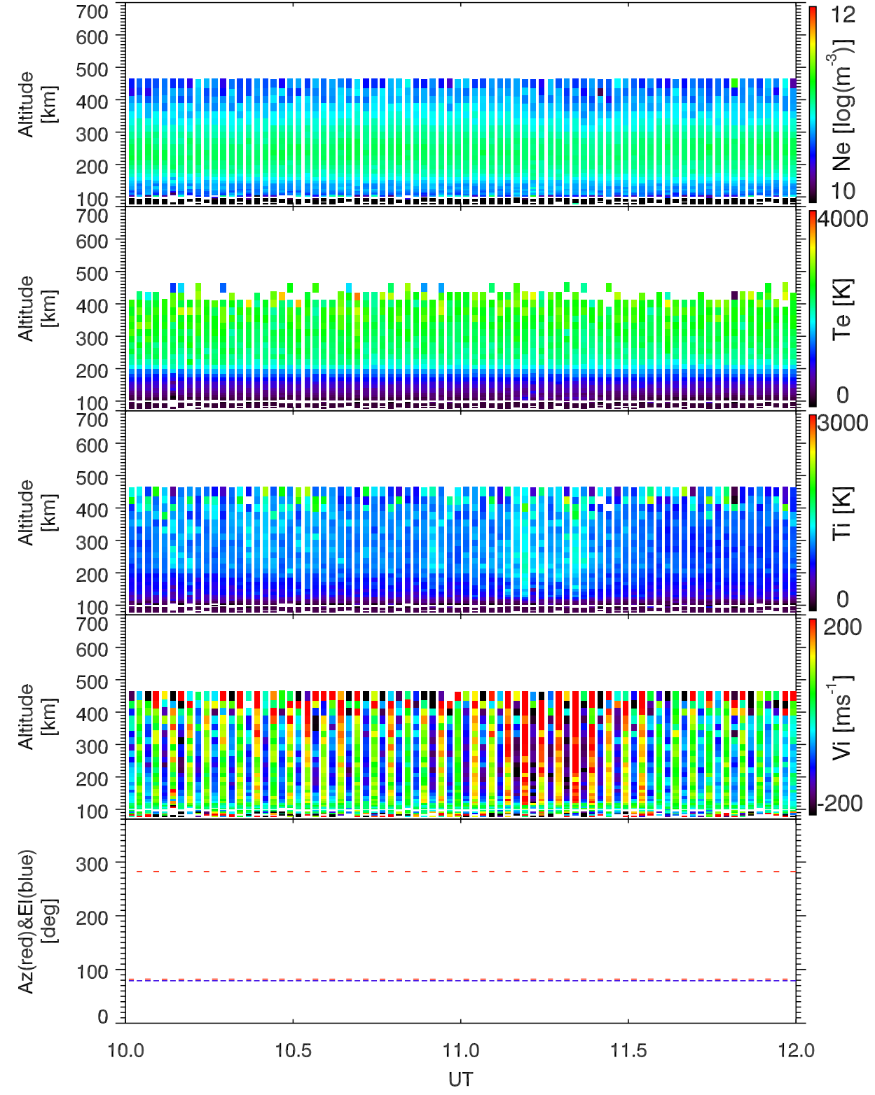
EISCAT 2007-04-04_10_12UT_ipy_ant@32m.
